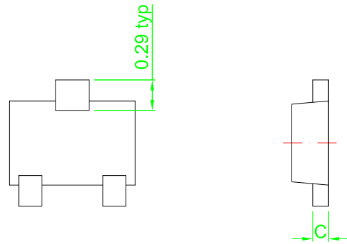
BTM SIDE
