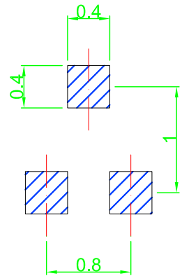
Recommended Land Pattern
