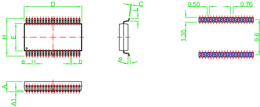
Recommended Land Pattern
