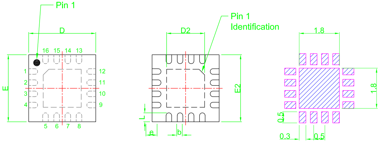
Recommended Land Pattern
