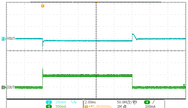
Load Transient
