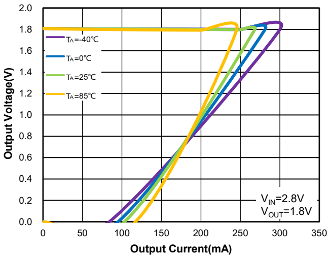
Figure 39. WR0331-18FF4R Foldback Current Limit vs. IOUT & Ambient Temperature
