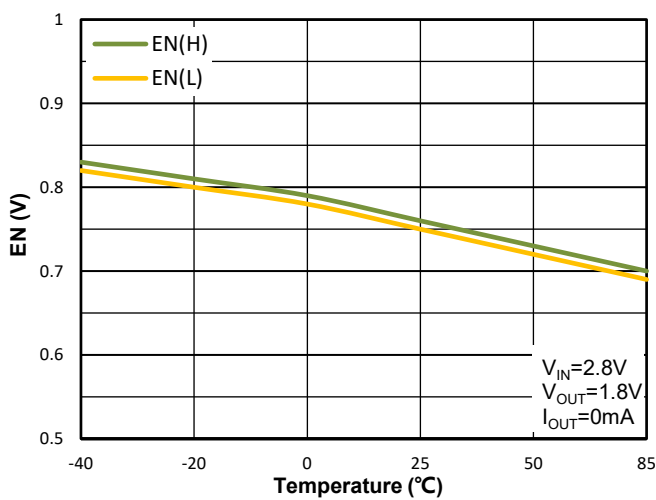
Figure 35. WR0331-18FF4R Enable Threshold vs. Ambient Temperature
