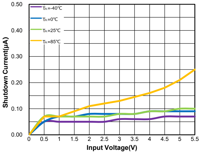
Figure 31. WR0331-18FF4R Shutdown Current vs. V IN & Ambient Temperature
