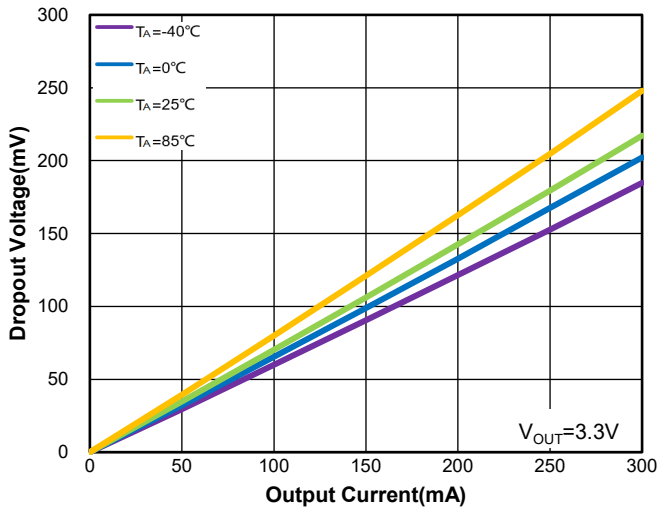
Figure 7. WR0331-33FF4R Dropout Voltage vs. I OUT & Ambient Temperature
