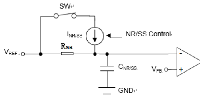
Soft-Start Circuit
