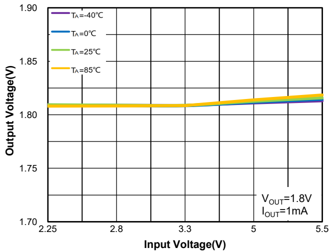
Figure9.WR0331-18FF4R Regulation vs. V IN (Line Regulation) & Ambient Temperature
