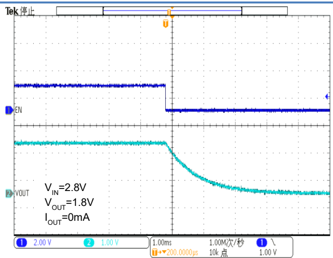
Figure 53. EN Shutdown
