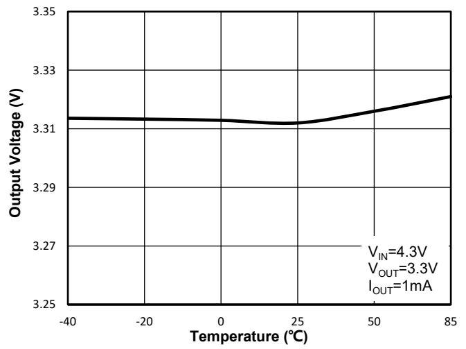
Figure 46. WR0331-33A50R Output Voltage vs. Ambient Temperature
