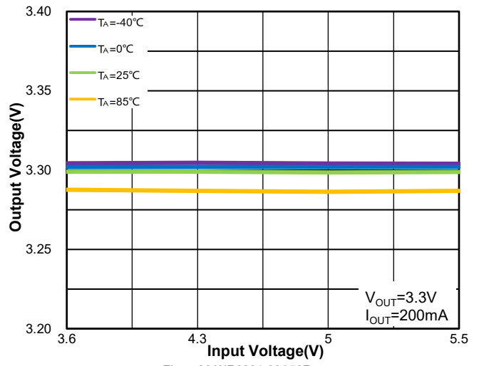
Figure20.WR0331-33A50R Regulation vs. V IN (Line Regulation) & Ambient Temperature
