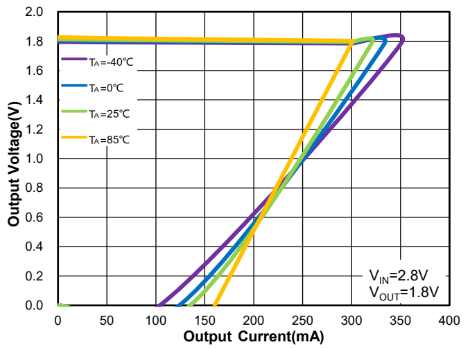
Figure 40. WR0331-18A50RR Foldback Current Limit vs. IOUT & Ambient Temperature
