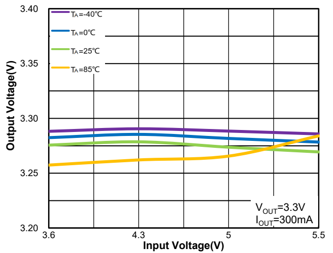
Figure22.WR0331-33A50R Regulation vs. V IN (Line Regulation) & Ambient Temperature
