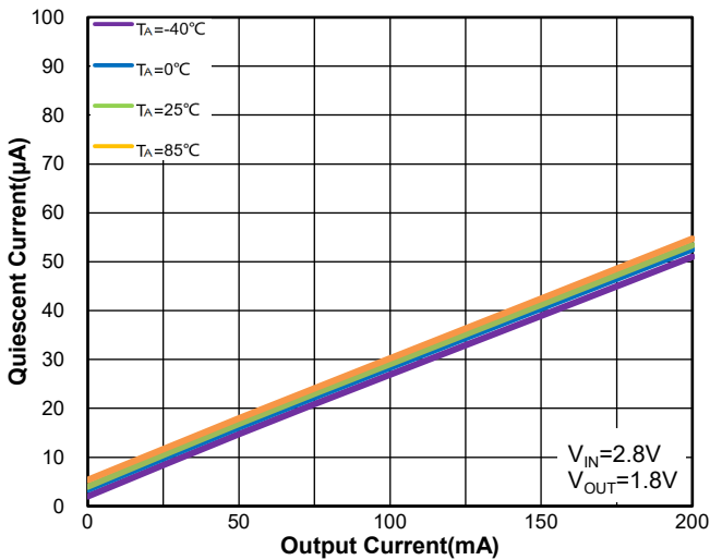
Figure23. WR0331-18FF4R Quiescent Current vs. I OUT & Ambient Temperature
