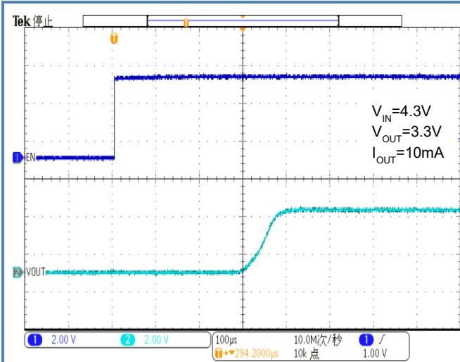
Figure 54. Soft Start from EN
