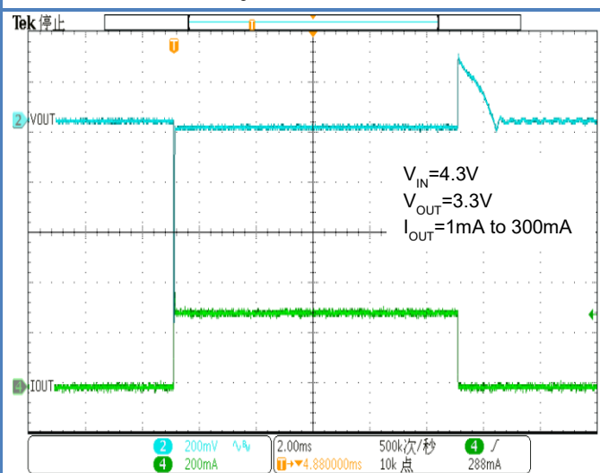
Figure 59. Load Transient
