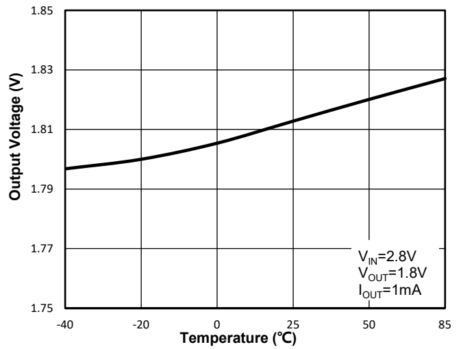
Figure 44. WR0331-18A50R Output Voltage vs. Ambient Temperature
