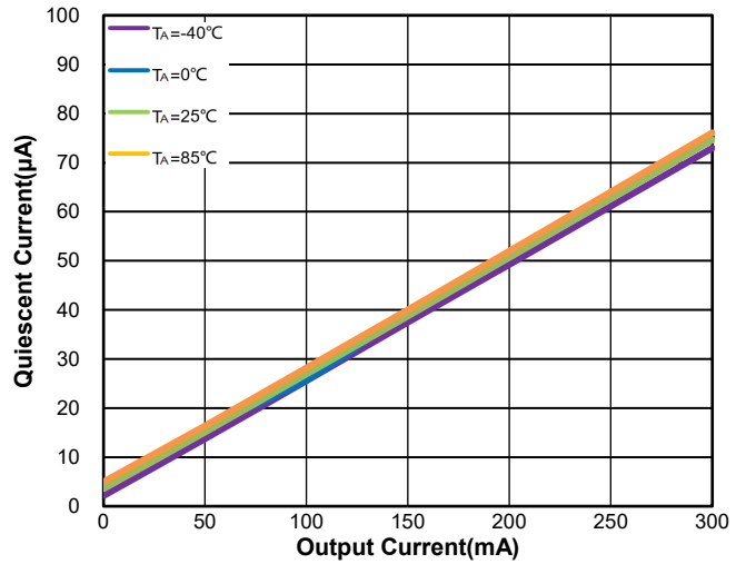
Figure 26. WR0331-33A50R Quiescent Current vs. I OUT & Ambient Temperature
