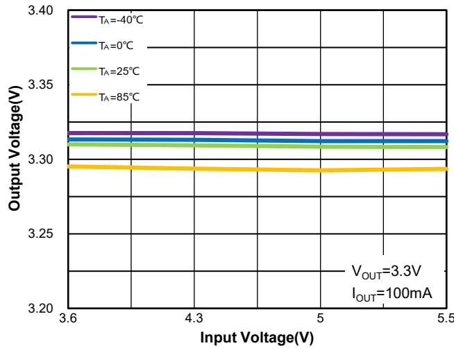
Figure 15.WR0331-33FF4R Regulation vs. V IN (Line Regulation) & Ambient Temperature
