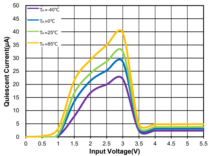
Figure 30. WR0331-3A50R Quiescent Current vs. V IN & Ambient Temperature
