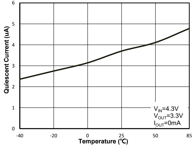
Figure 50. WR0331-33A50R Quiescent Current vs. Ambient Temperature
