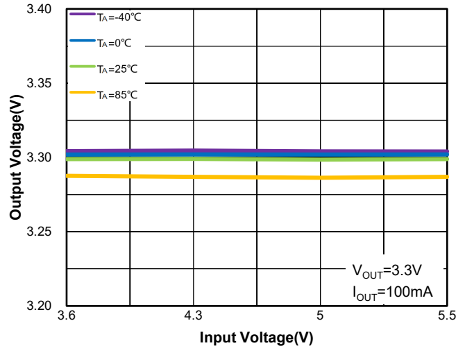
Figure 16.WR0331-33A50R Regulation vs. V IN (Line Regulation) & Ambient Temperature
