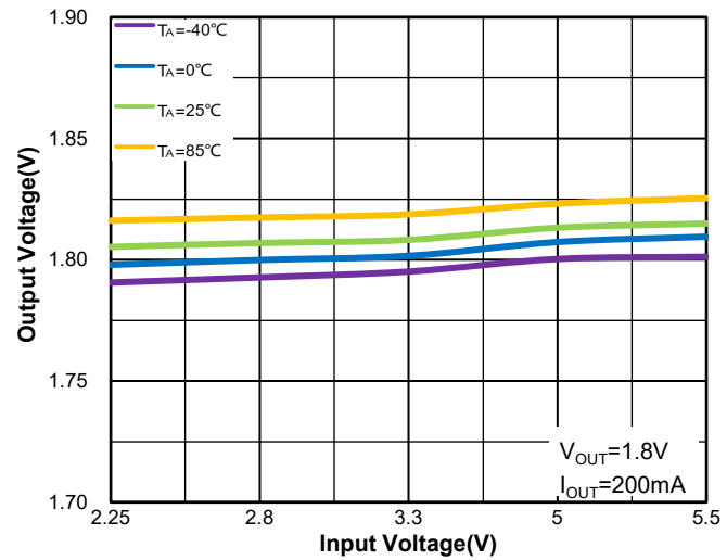
Figure 18.WR0331-18A50R Regulation vs. V IN (Line Regulation) & Ambient Temperature
