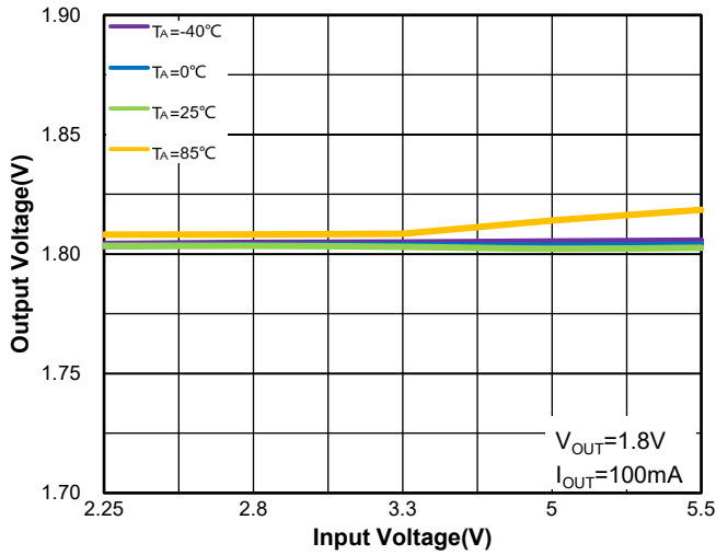
Figure 13.WR0331-18FF4R Regulation vs. V IN (Line Regulation) & Ambient Temperature
