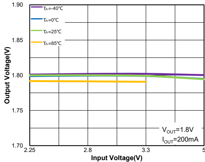
Figure 17.WR0331-18FF4R Regulation vs. V IN (Line Regulation) & Ambient Temperature
