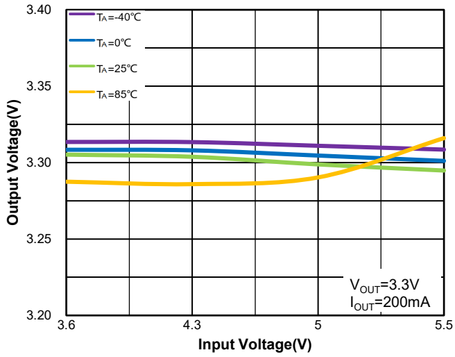
Figure19.WR0331-33FF4R Regulation vs. V IN (Line Regulation) & Ambient Temperature
