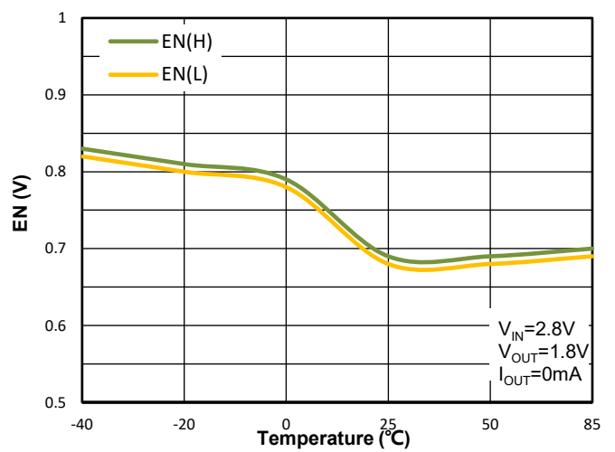
Figure 36. WR0331-18A50R Enable Threshold vs. Ambient Temperature
