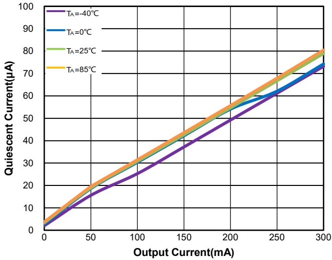
Figure 25. WR0331-33FF4R Quiescent Current vs. I OUT & Ambient Temperature
