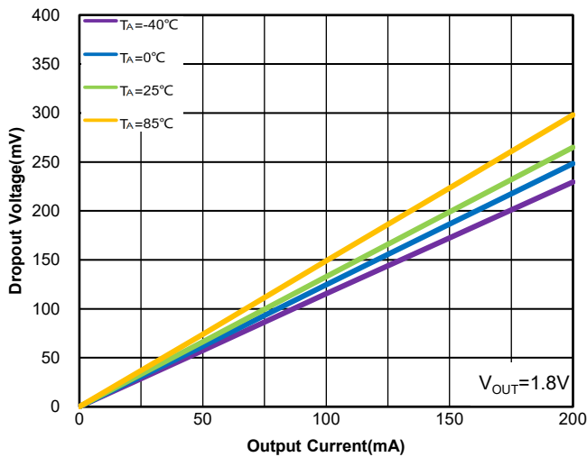
Figure 5. WR0331-18FF4R Dropout Voltage vs. I OUT & Ambient Temperature
