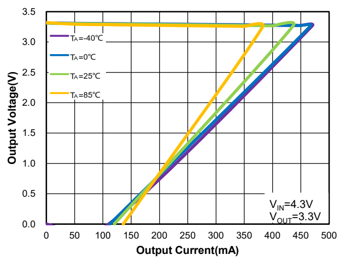
Figure 42. WR0331-33A50R Foldback Current Limit vs. IOUT & Ambient Temperature
