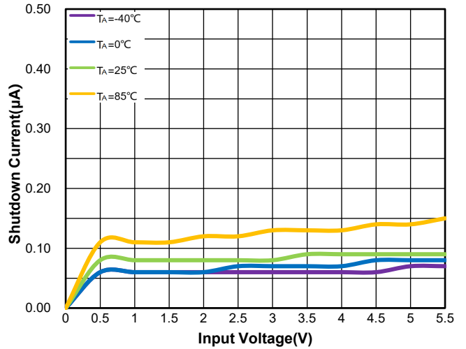
Figure 32. WR0331-18A50R Shutdown Current vs. V IN & Ambient Temperature
