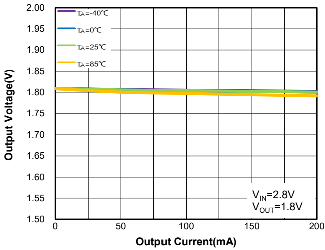
Figure 1. WR0331-18FF4R Load Regulation vs. I OUT & Ambient Temperature
