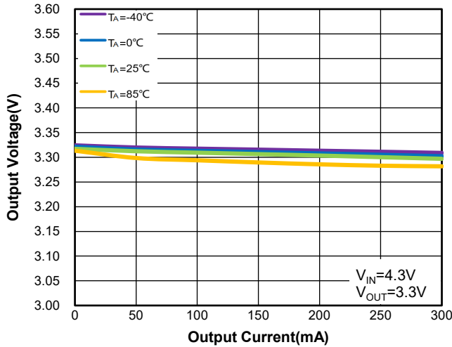
Figure 3. WR0331-33FF4R Load Regulation vs. I OUT & Ambient Temperature
