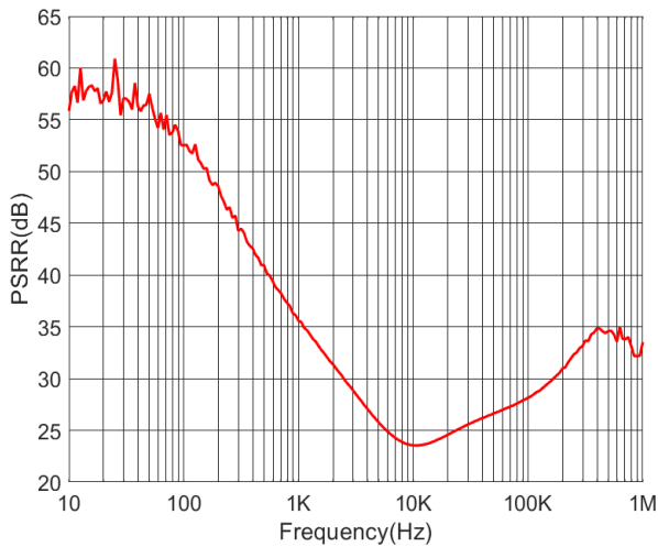
Figure 51. Power Supply Rejection Ratio vs. Frequency
