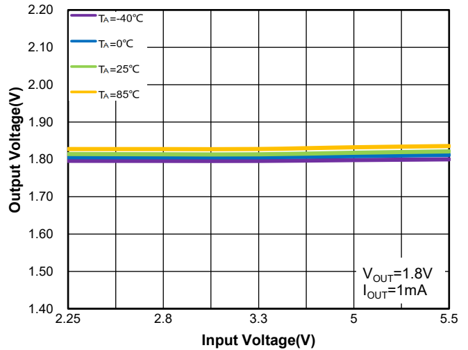
Figure10.WR0331-18A50R Regulation vs. V IN (Line Regulation) & Ambient Temperature
