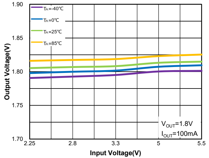
Figure 14.WR0331-18A50R Regulation vs. V IN (Line Regulation) & Ambient Temperature
