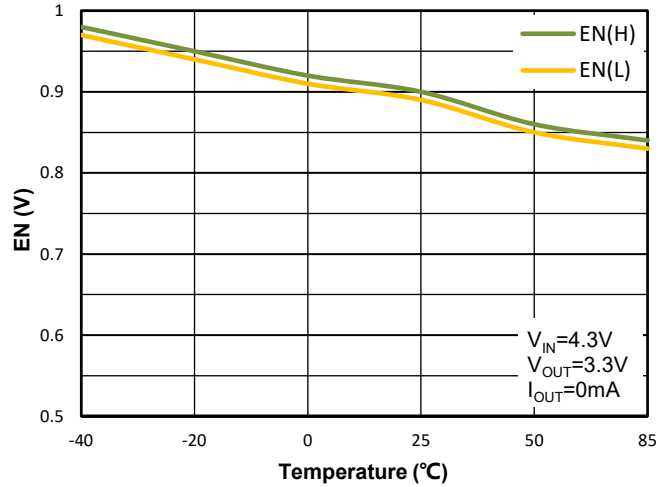
Figure 38. WR0331-33A50R Enable Threshold vs. Ambient Temperature
