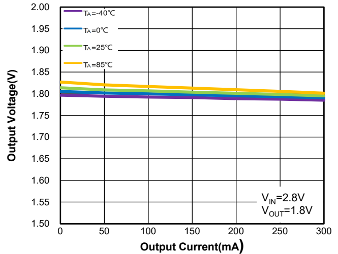
Figure 2. WR0331-18A50R Load Regulation vs. I OUT & Ambient Temperature
