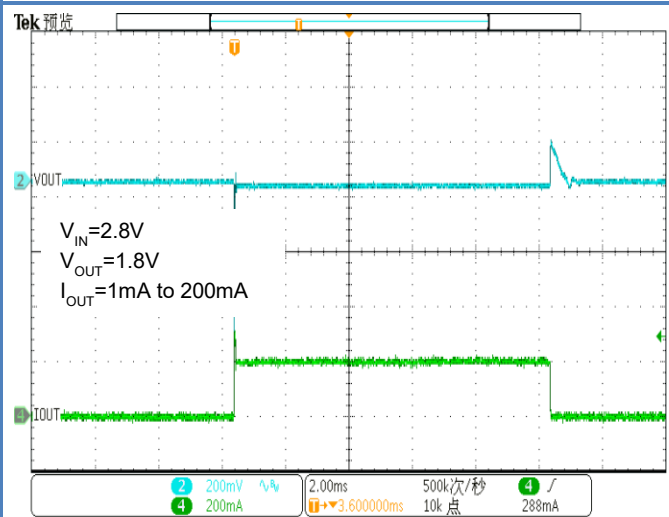
Figure 57. Load Transient
