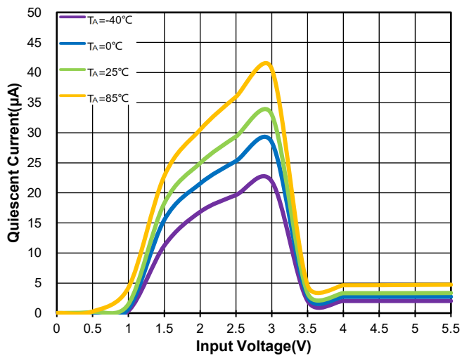
Figure 29. WR0331-33FF4R Quiescent Current vs. V IN & Ambient Temperature
