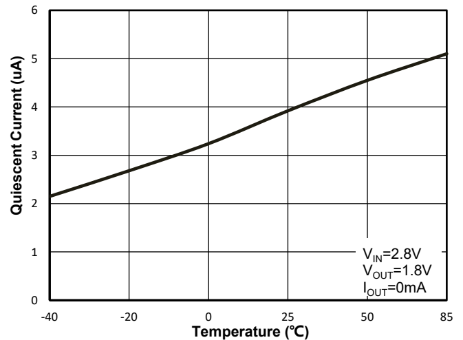
Figure 48. WR0331-18A50R Quiescent Current vs. Ambient Temperature
