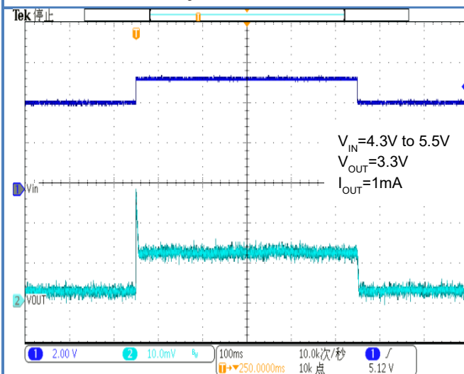
Figure 58. Line Transient
