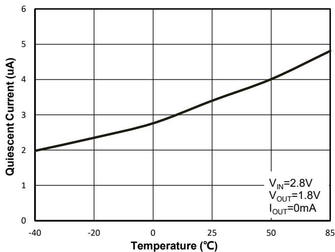
Figure 47. WR0331-18FF4R Quiescent Current vs. Ambient Temperature
