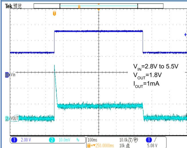
Figure 56. Line Transient
