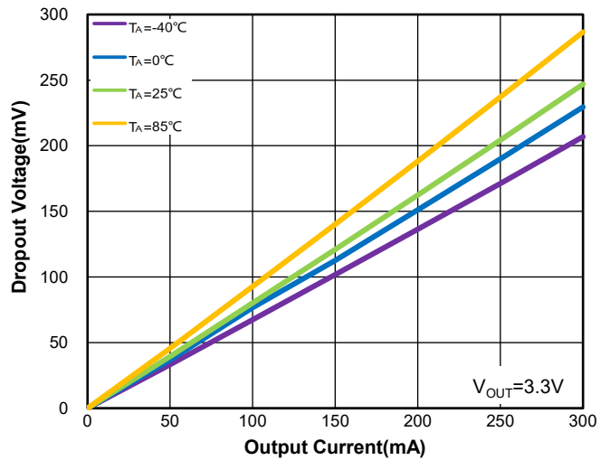
Figure 8. WR0331-33A50R Dropout Voltage vs. I OUT & Ambient Temperature
