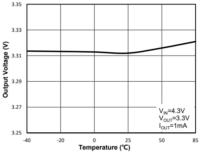
Figure 45. WR0331-33FF4R Output Voltage vs. Ambient Temperature
