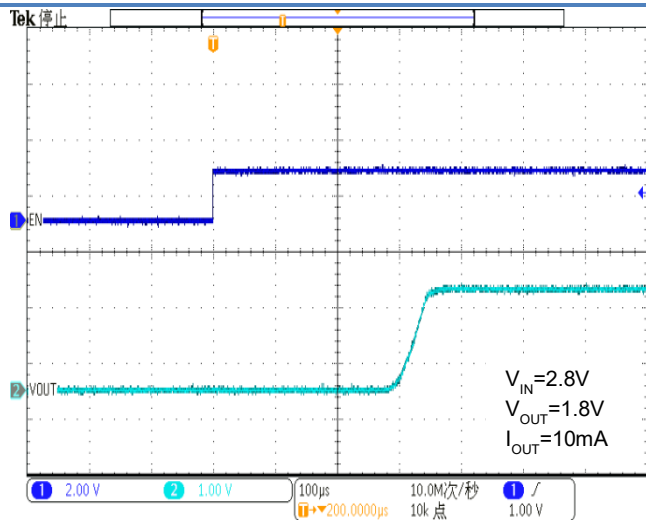
Figure 52. Soft Start from EN
