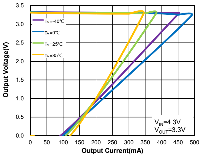
Figure 41. WR0331-33FF4R Foldback Current Limit vs. IOUT & Ambient Temperature
