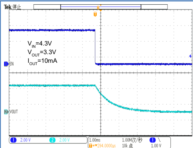
Figure 55. EN Shutdown
