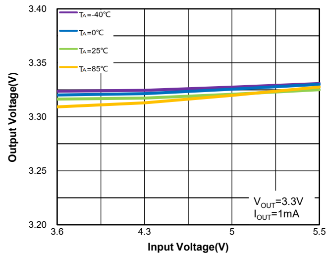
Figure11.WR0331-33FF4R Regulation vs. V IN (Line Regulation) & Ambient Temperature
