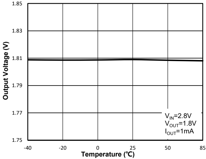
Figure 43. WR0331-18FF4R Output Voltage vs. Ambient Temperature
