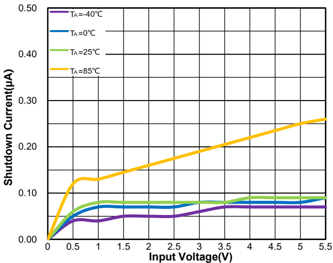
Figure 33. WR0331-33FF4R Shutdown Current vs. V IN & Ambient Temperature
