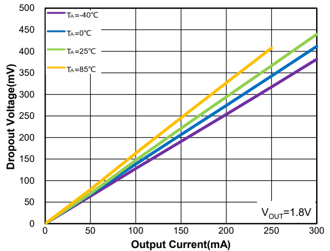
Figure 6. WR0331-18A50R Dropout Voltage vs. I OUT & Ambient Temperature
