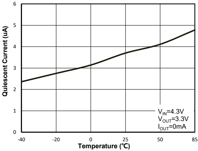
Figure 49. WR0331-33FF4R Quiescent Current vs. Ambient Temperature
