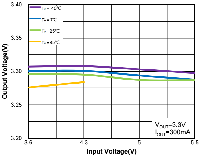
Figure21.WR0331-33FF4R Regulation vs. V IN (Line Regulation) & Ambient Temperature
