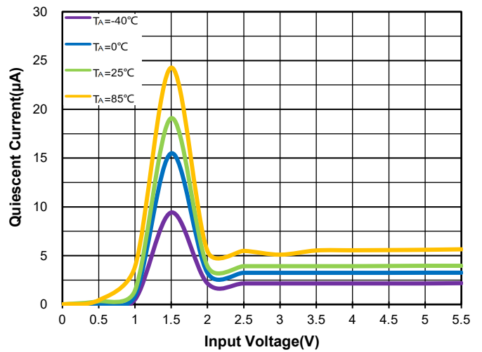
Figure 28. WR0331-18A50R Quiescent Current vs. V IN & Ambient Temperature
