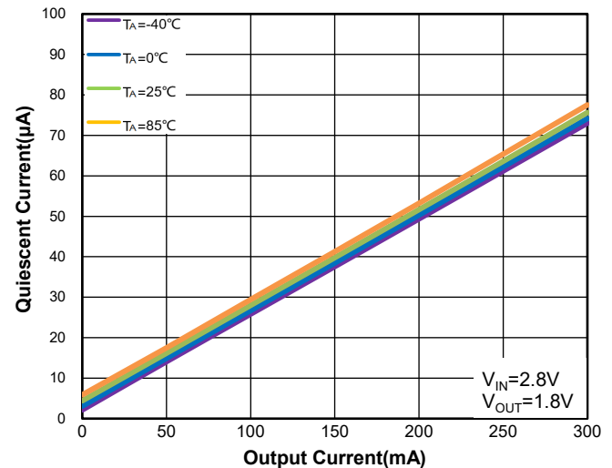
Figure24. WR0331-18A50R Quiescent Current vs. I OUT & Ambient Temperature
