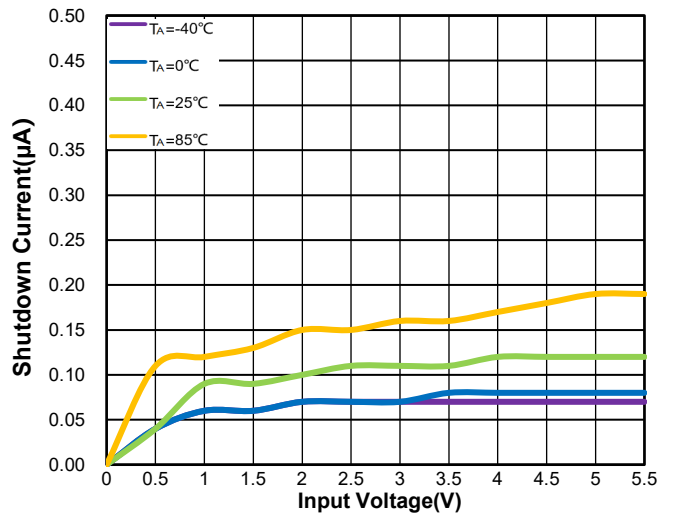
Figure 34. WR0331-33A50R Shutdown Current vs. V IN & Ambient Temperature
