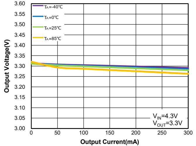
Figure 4. WR0331-33A50R Load Regulation vs. I OUT & Ambient Temperature
