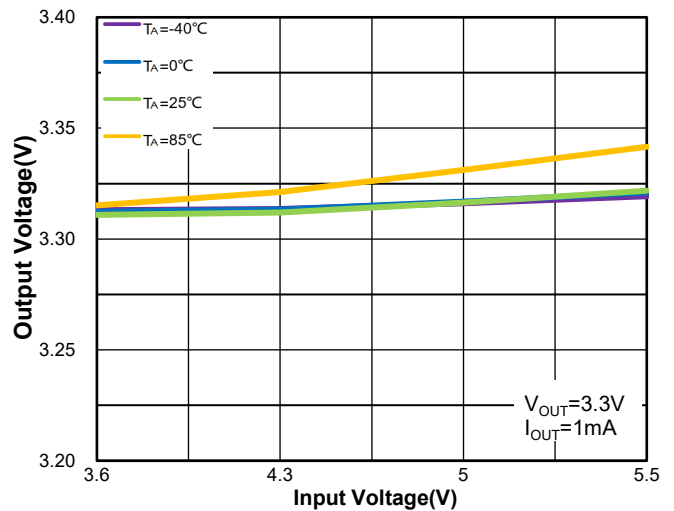
Figure12.WR0331-33A50R Regulation vs. V IN (Line Regulation) & Ambient Temperature
