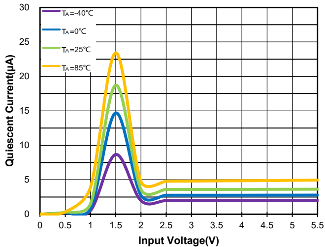
Figure 27. WR0331-18FF4R Quiescent Current vs. V IN & Ambient Temperature
