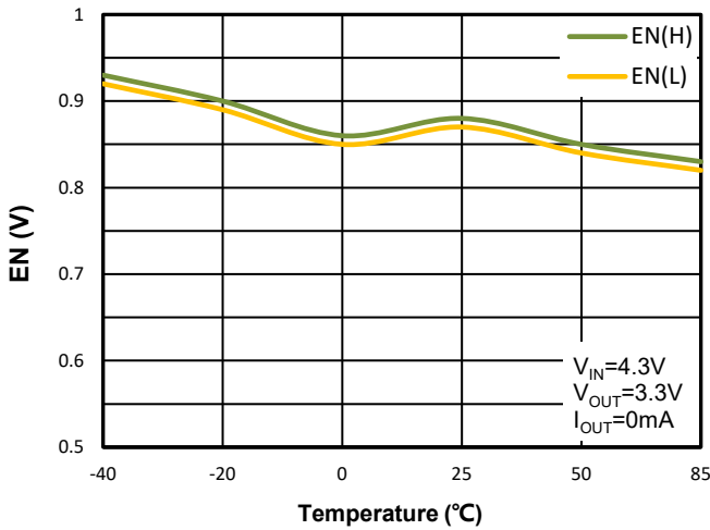
Figure 37. WR0331-33FF4R Enable Threshold vs. Ambient Temperature
