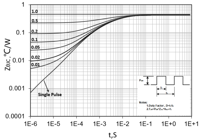
Figure 10. Transient Thermal Response Curve (TO-247)
