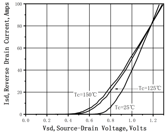
Figure 4. Typical Body Diode Transfer Characteristics
