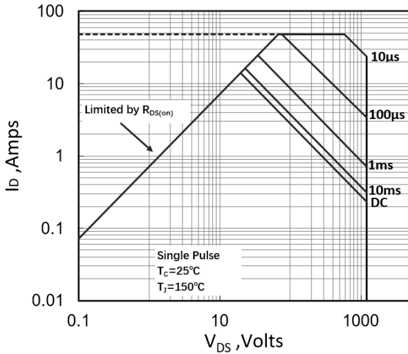
Figure 9. Maximum Safe Operating Area (TO-247)
