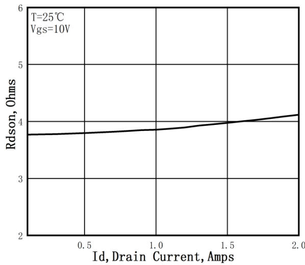
Figure 3. Static Drain-Source On Resistance
