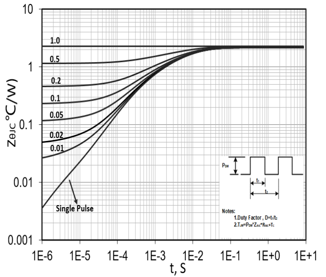
Figure 10. Transient Thermal Response Curve
