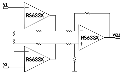
Figure 11. Amplifier instrumentation amplifier
