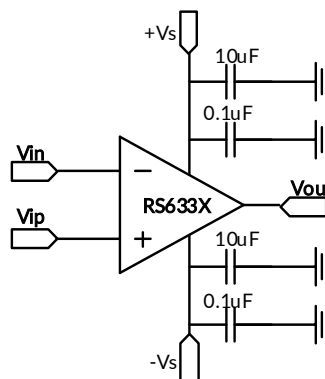
Figure 10. Amplifier with Bypass Capacitors
