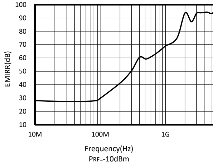
Figure 2. RS62XP EMIRR vs Frequency
