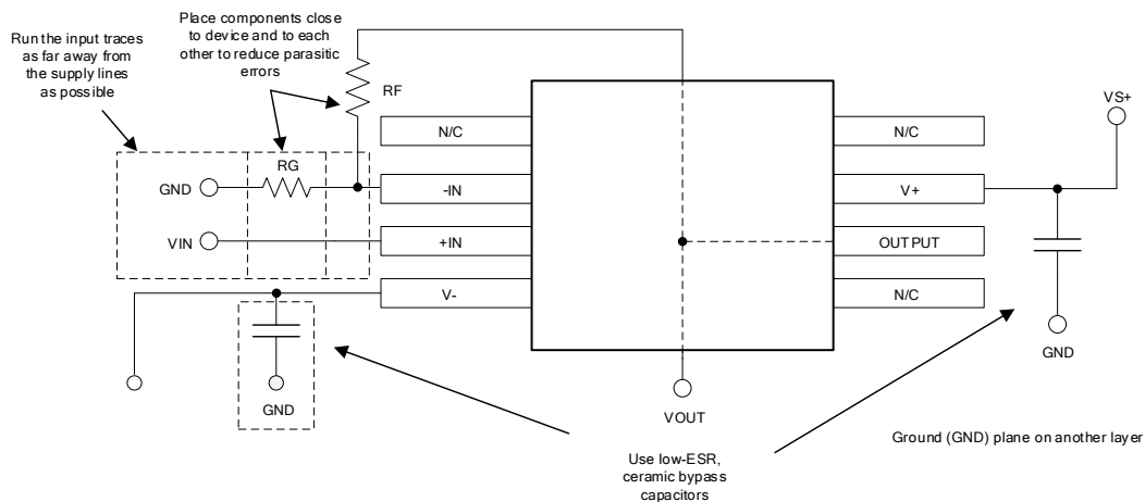
Figure 7. Operational Amplifier Board Layout for Noninverting Configuration
