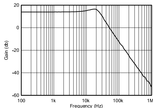
Figure 5. Low-pass filter transfer function
