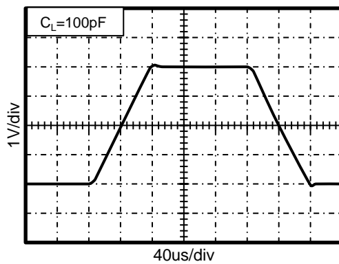
Figure 9. Large-Signal Step Response
