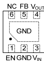
DFN1616-6 (TOP VIEW)
