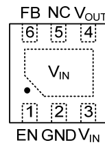
DFN2020-6 (TOP VIEW)
