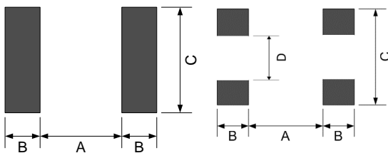
PCB Solder Pad
