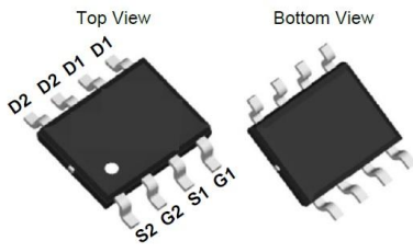
SOP-8(Dual)
