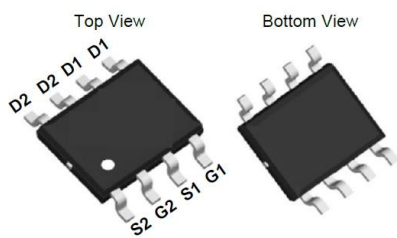
SOP-8(Dual)
