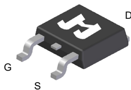
TO-252-3L Top View
