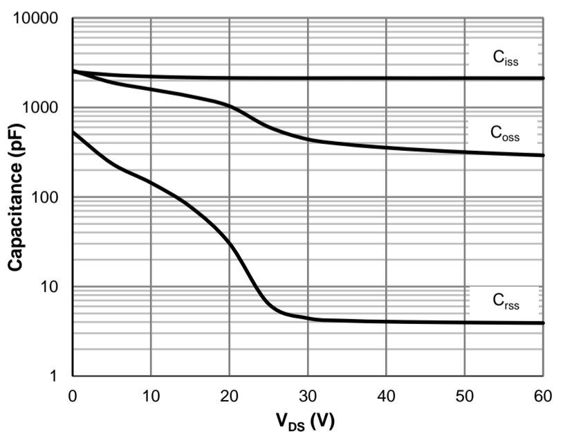
Figure 6: Capacitance Characteristics
