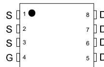
Pin Configuration Top View
