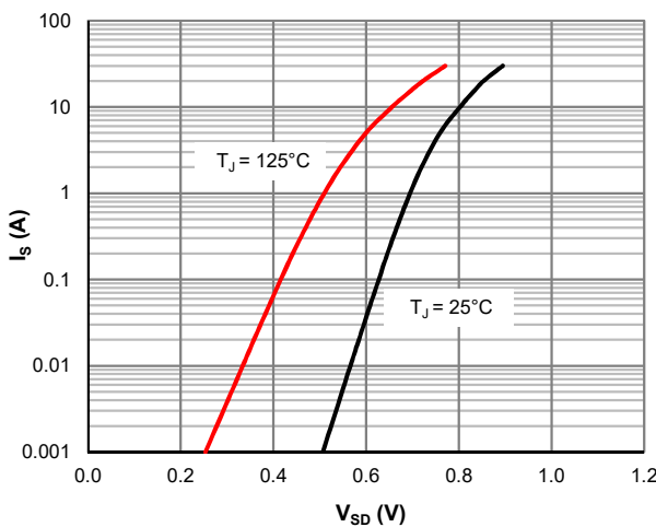
Figure 5: Body-Diode Characteristics
