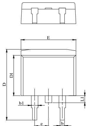
Package Outline
