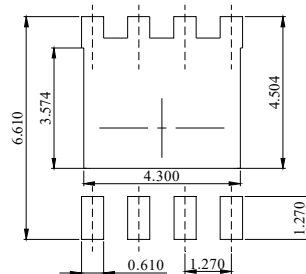
DIMENSIONS: MILLIMETERS
