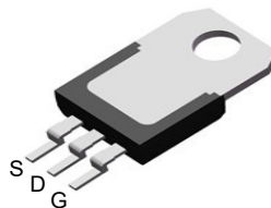
TO220AS Bottom View
