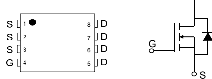
Pin Configuration Top View
